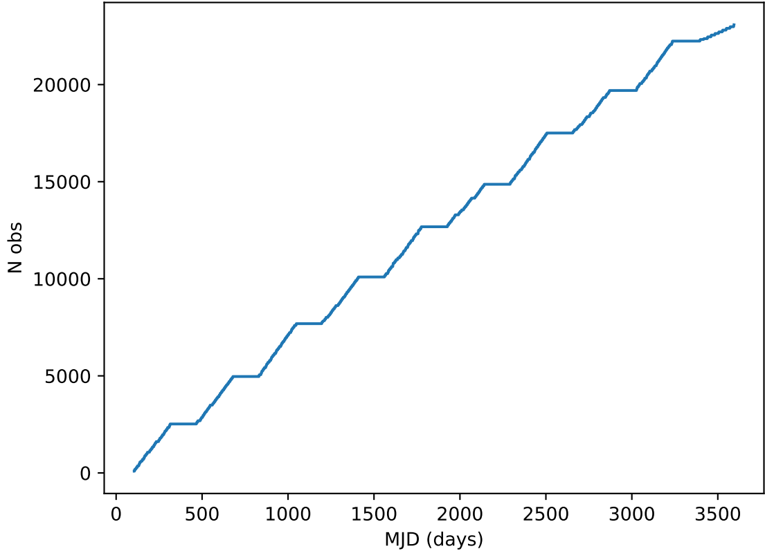
roll_uniform_eh_acc1.0_mjdp0_v3.4_10yrs all bands: DD:EDFS Cumulative NVisits
