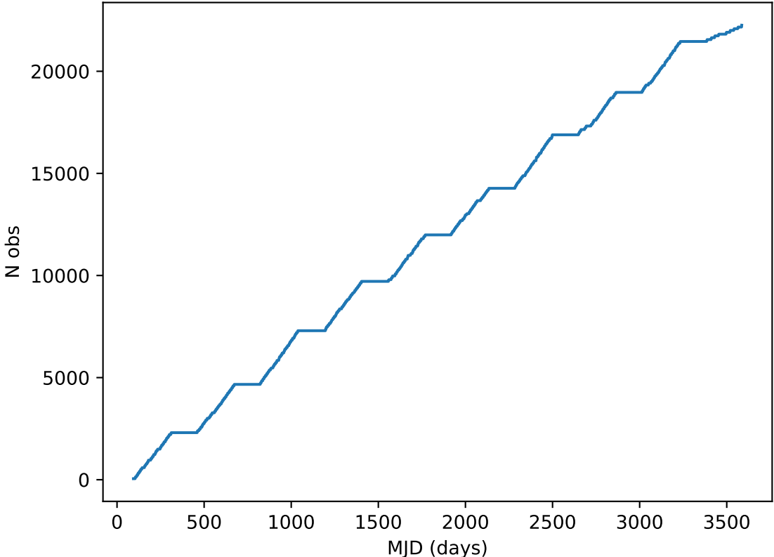
roll_uniform_eh_acc1.0_mjdp0_v3.4_10yrs all bands: DD:ECDFS Cumulative NVisits
