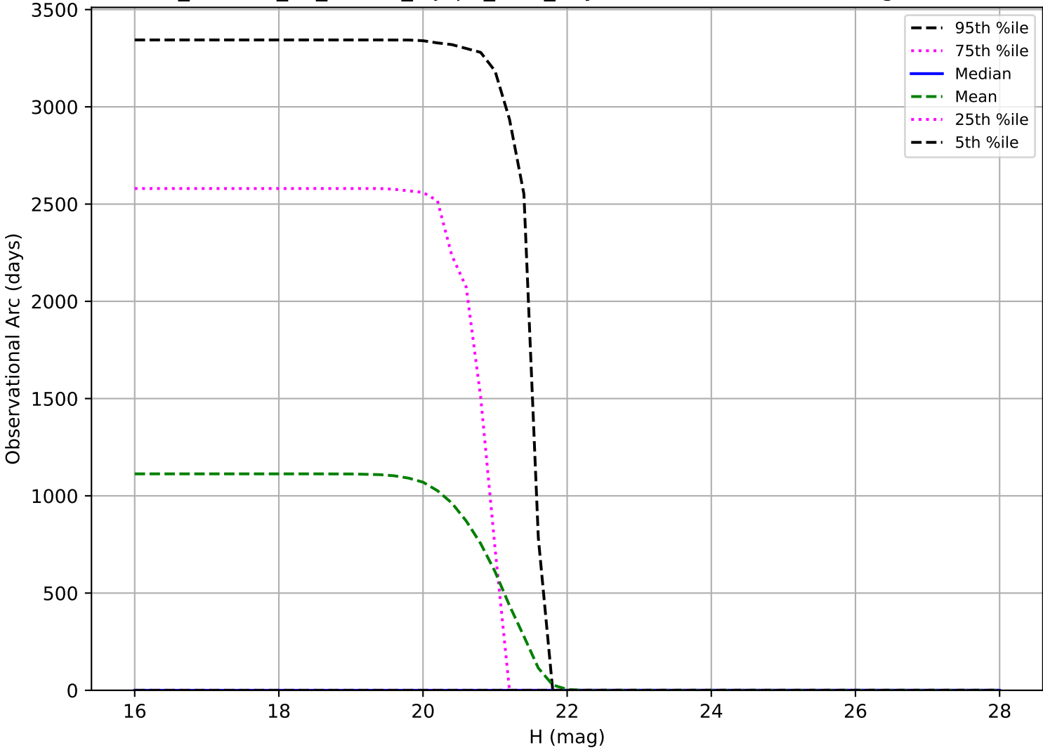
roll_uniform_eh_acc0.8_mjdp0_v3.4_10yrs: Observational Arc Length Vatira
