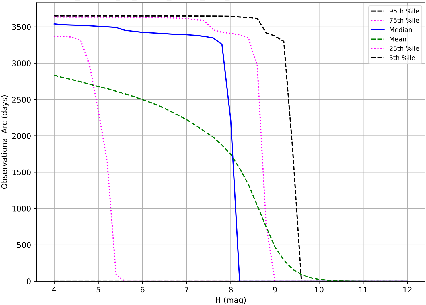
roll_uniform_eh_acc0.8_mjdp0_v3.4_10yrs: Observational Arc Length TNO
