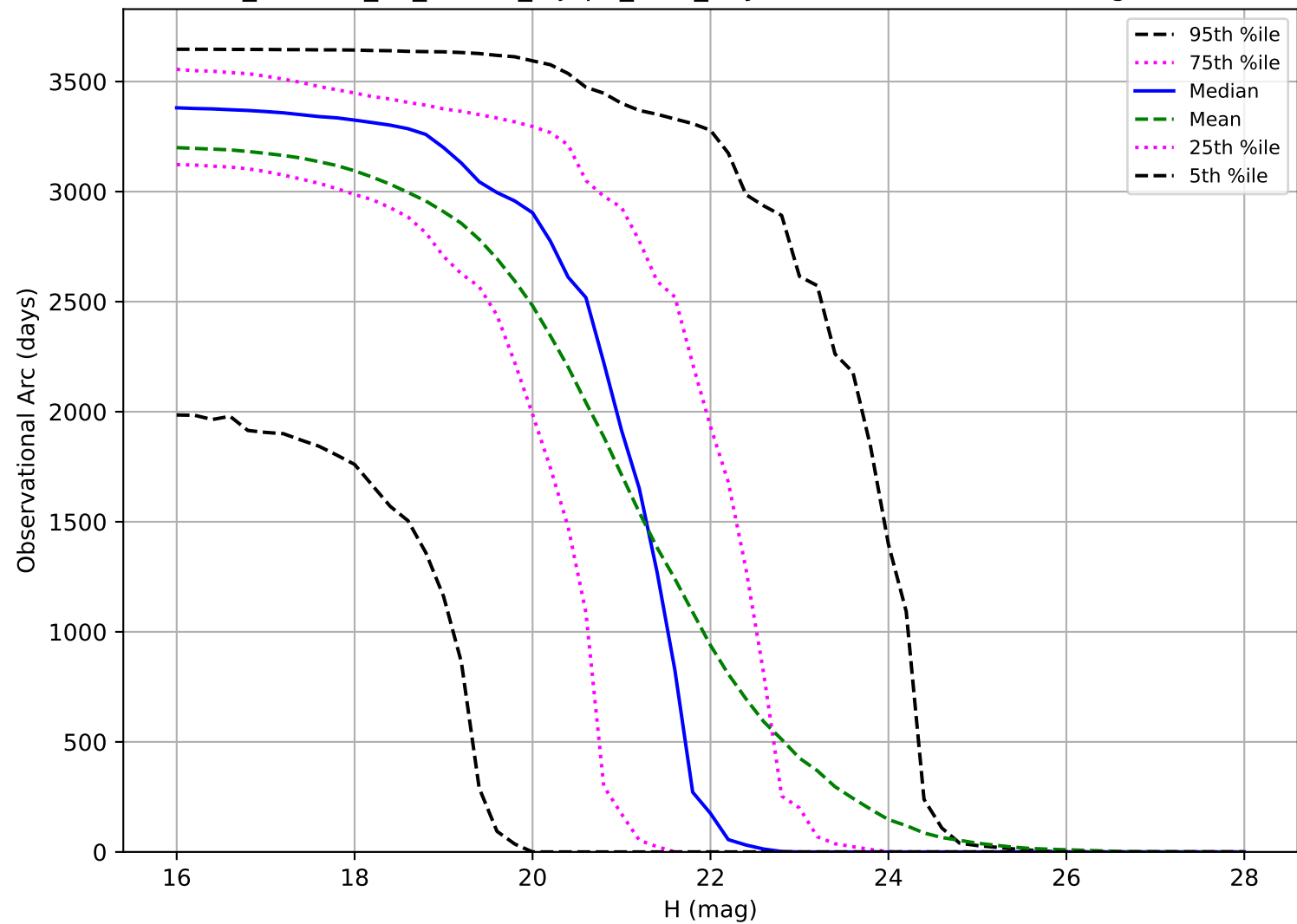
roll_uniform_eh_acc0.8_mjdp0_v3.4_10yrs: Observational Arc Length PHA
