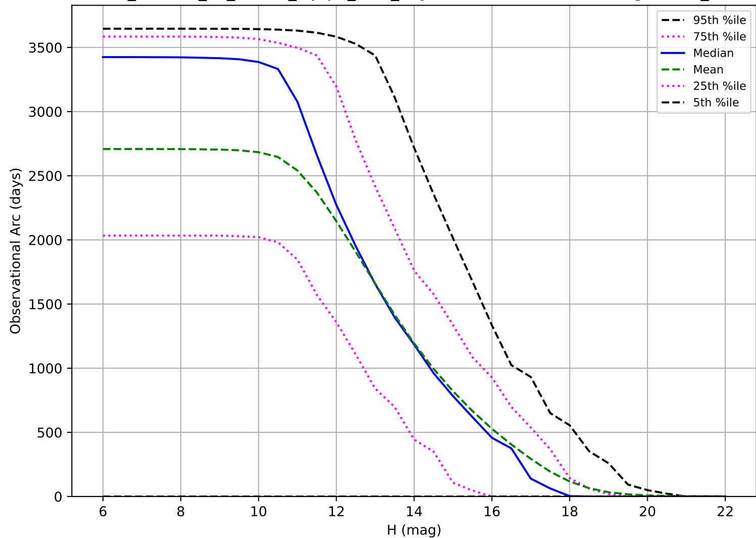
roll_uniform_eh_acc0.8_mjdp0_v3.4_10yrs: Observational Arc Length OCC_r5
