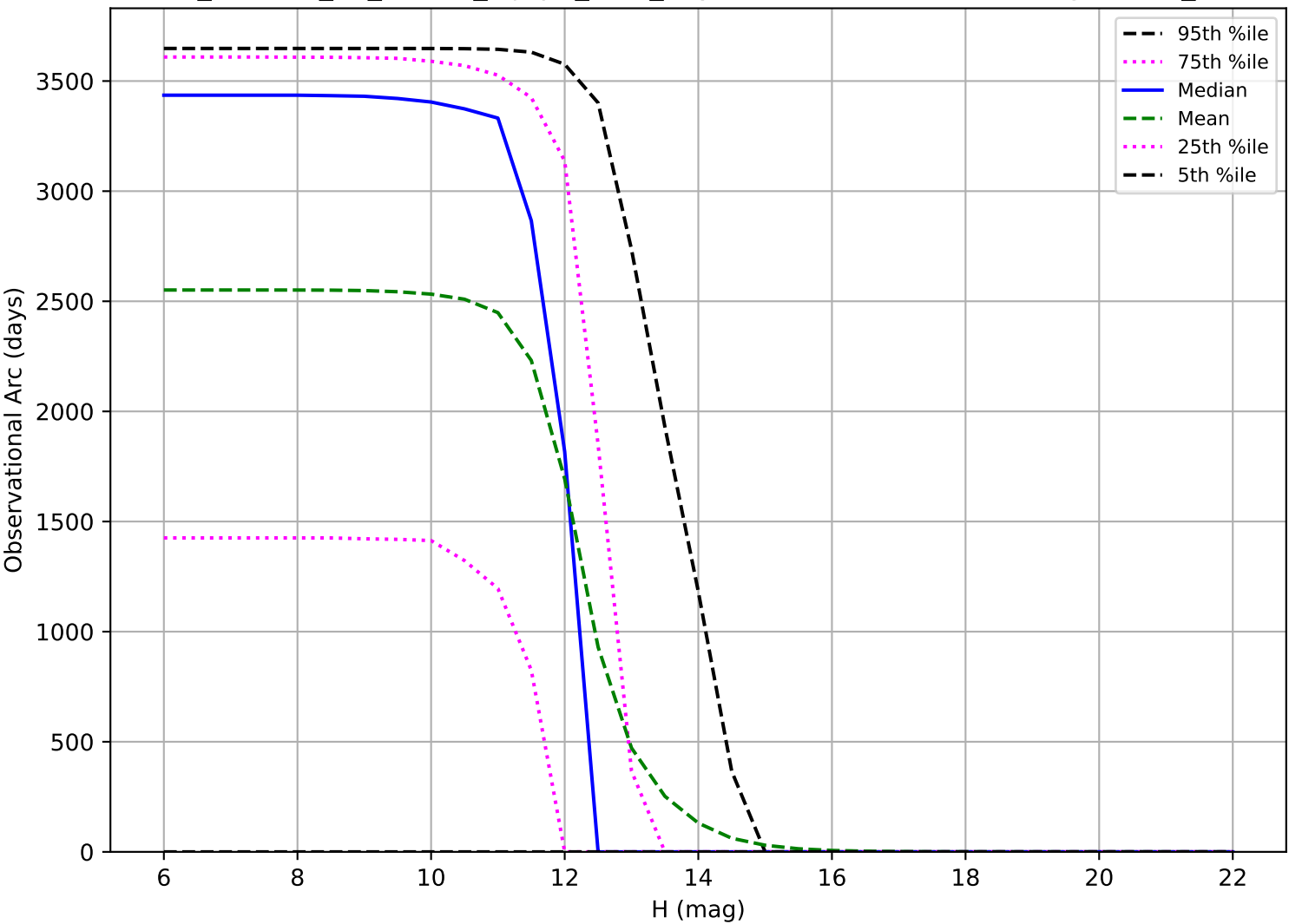
roll_uniform_eh_acc0.8_mjdp0_v3.4_10yrs: Observational Arc Length OCC_r20
