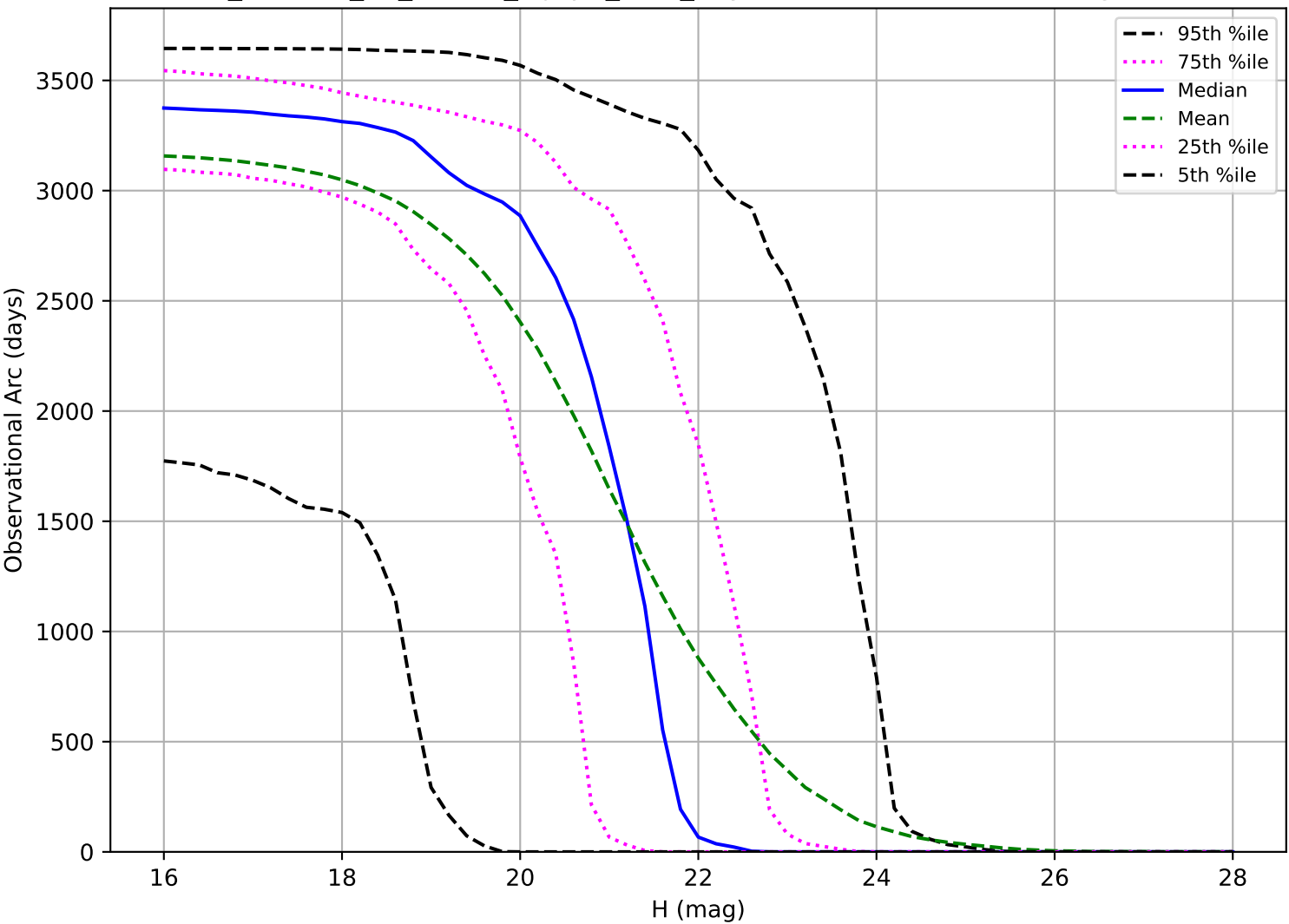
roll_uniform_eh_acc0.8_mjdp0_v3.4_10yrs: Observational Arc Length NEO
