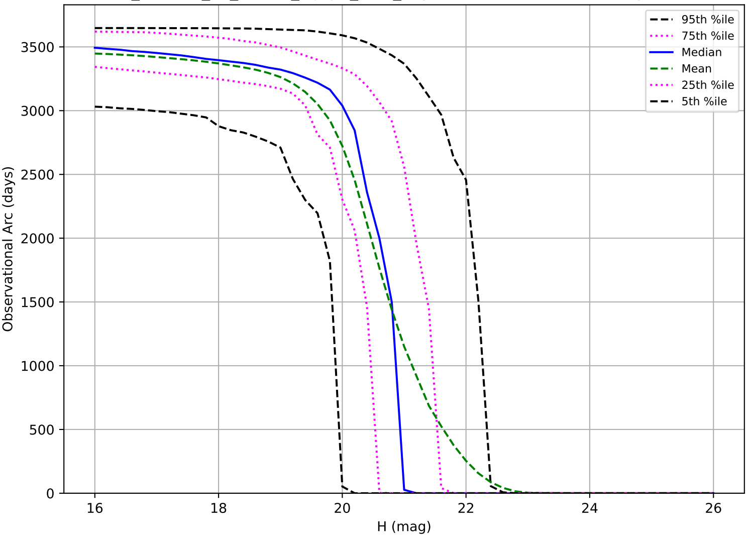
roll_uniform_eh_acc0.8_mjdp0_v3.4_10yrs: Observational Arc Length MBA
