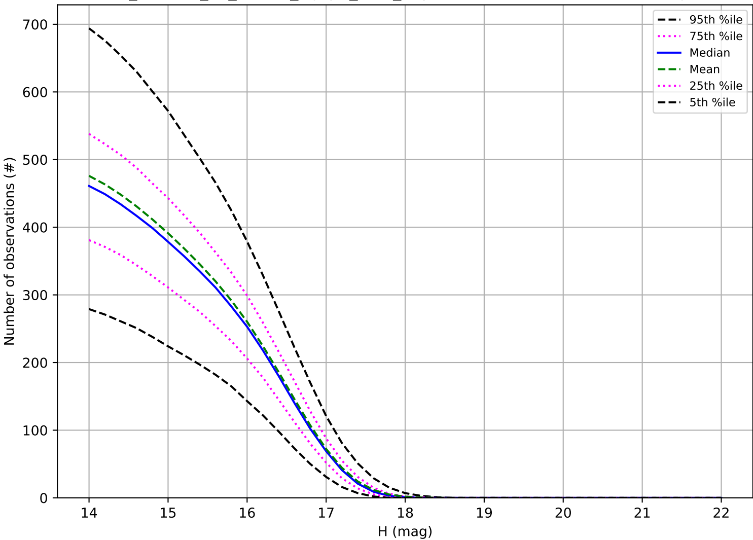
roll_uniform_eh_acc0.8_mjdp0_v3.4_10yrs: Number of observations Trojan
