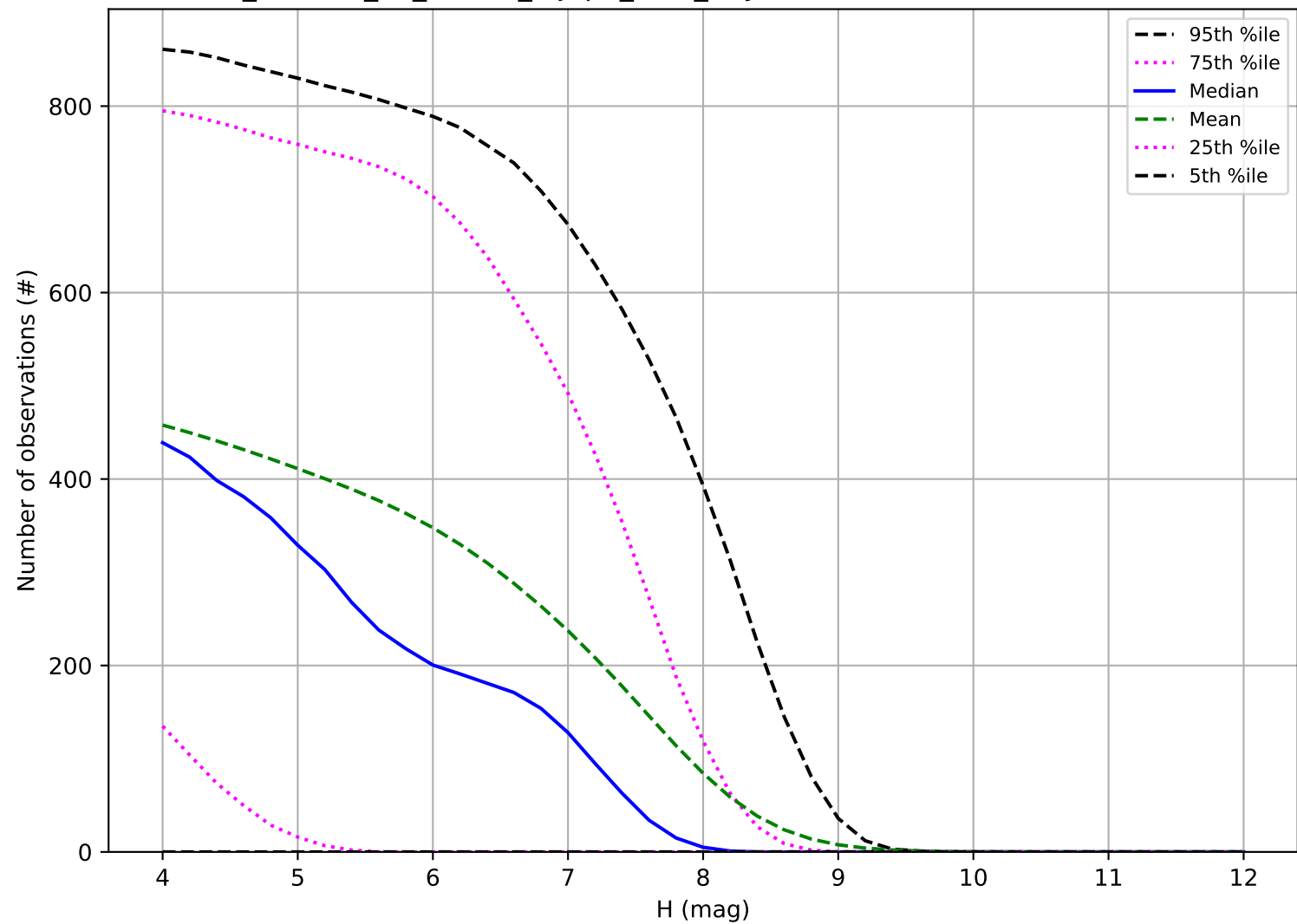
roll_uniform_eh_acc0.8_mjdp0_v3.4_10yrs: Number of observations TNO
