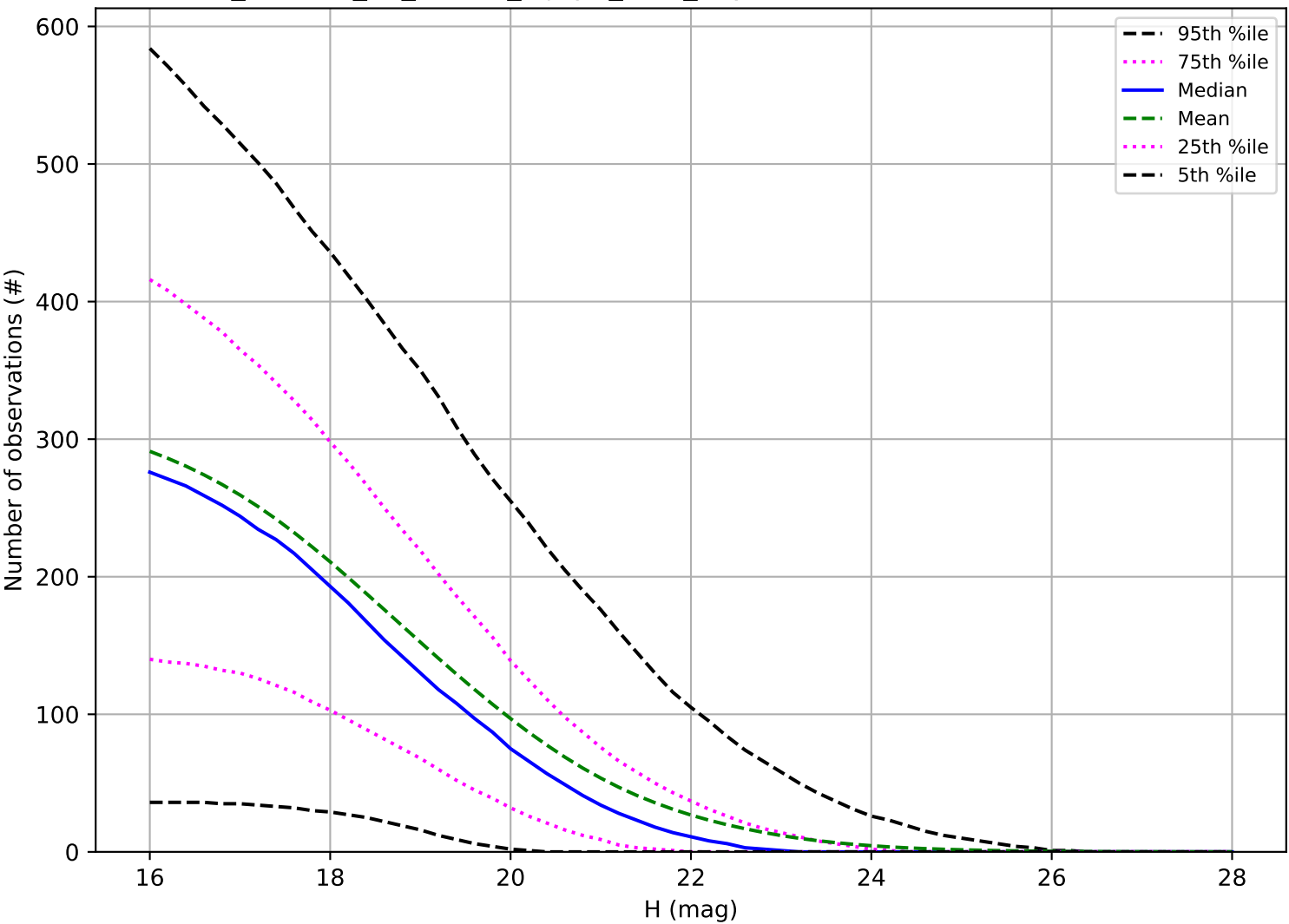
roll_uniform_eh_acc0.8_mjdp0_v3.4_10yrs: Number of observations PHA
