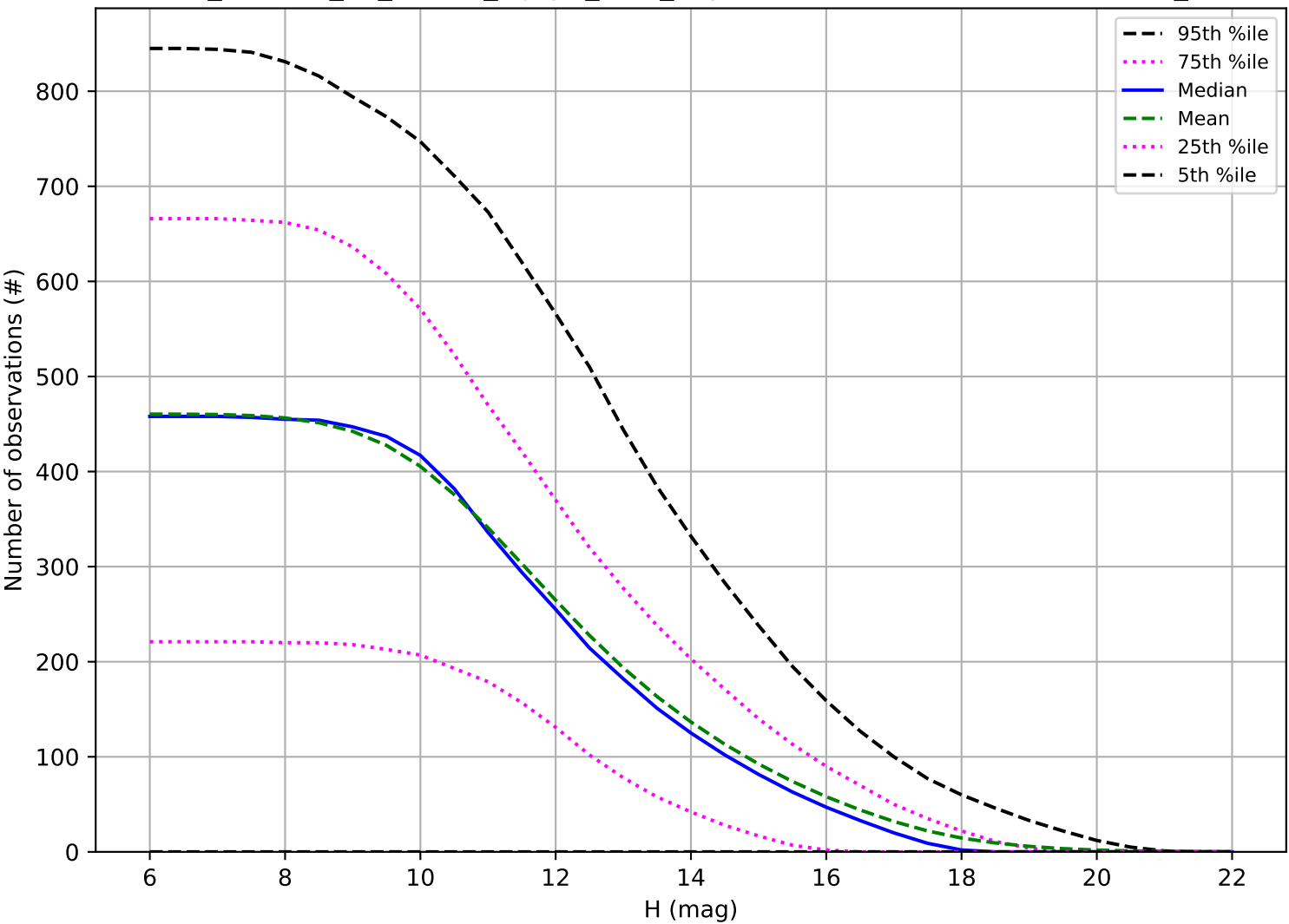
roll_uniform_eh_acc0.8_mjdp0_v3.4_10yrs: Number of observations OCC_r5
