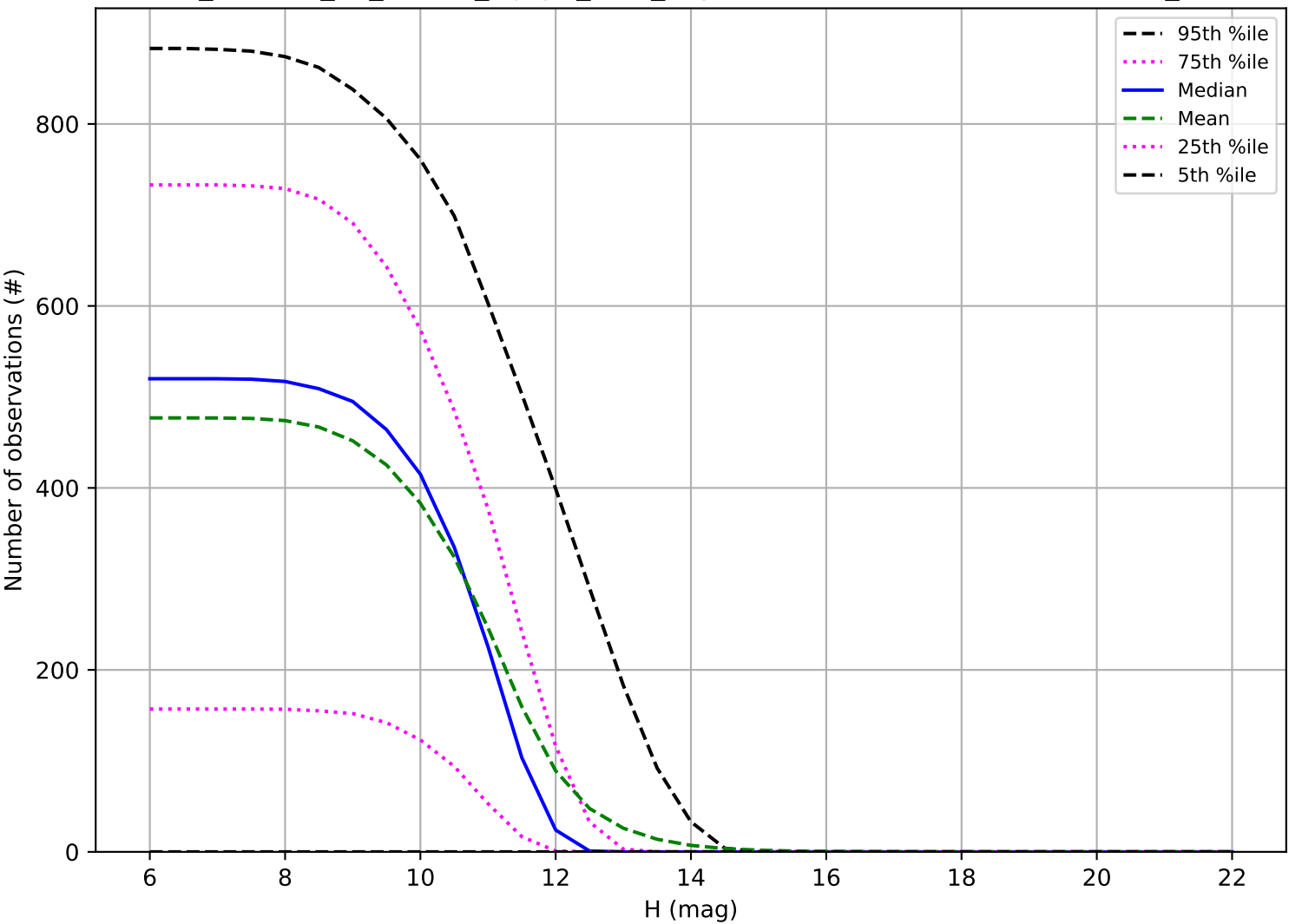
roll_uniform_eh_acc0.8_mjdp0_v3.4_10yrs: Number of observations OCC_r20
