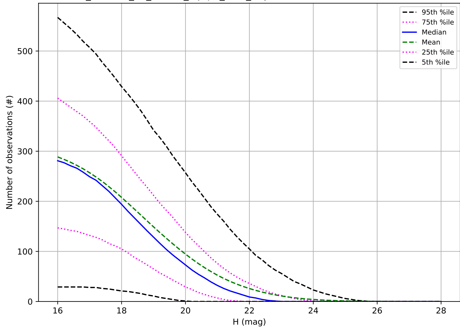
roll_uniform_eh_acc0.8_mjdp0_v3.4_10yrs: Number of observations NEO
