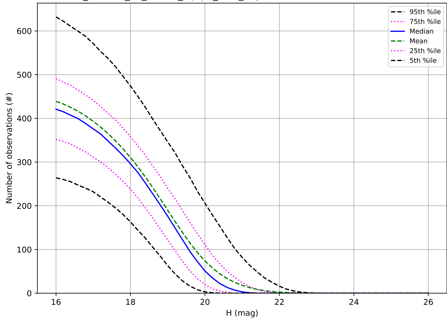
roll_uniform_eh_acc0.8_mjdp0_v3.4_10yrs: Number of observations MBA
