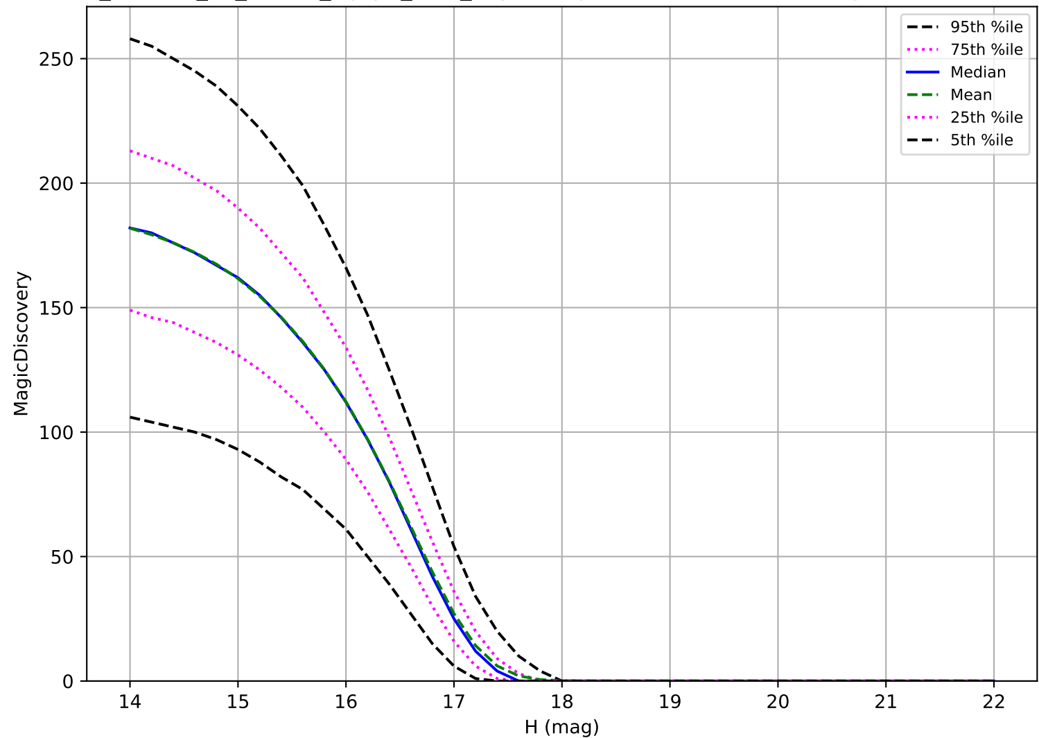
roll_uniform_eh_acc0.8_mjdp0_v3.4_10yrs: Trojan 6 detections in 60 nights detection loss
