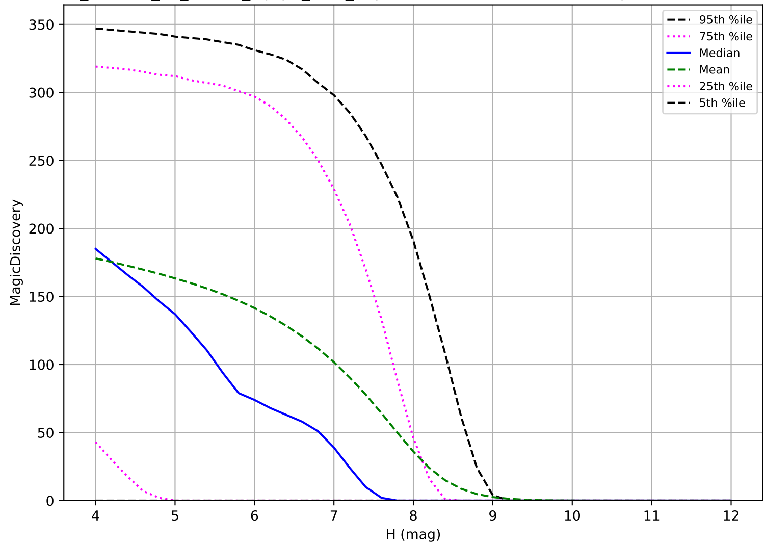
roll_uniform_eh_acc0.8_mjdp0_v3.4_10yrs: TNO 6 detections in 60 nights detection loss
