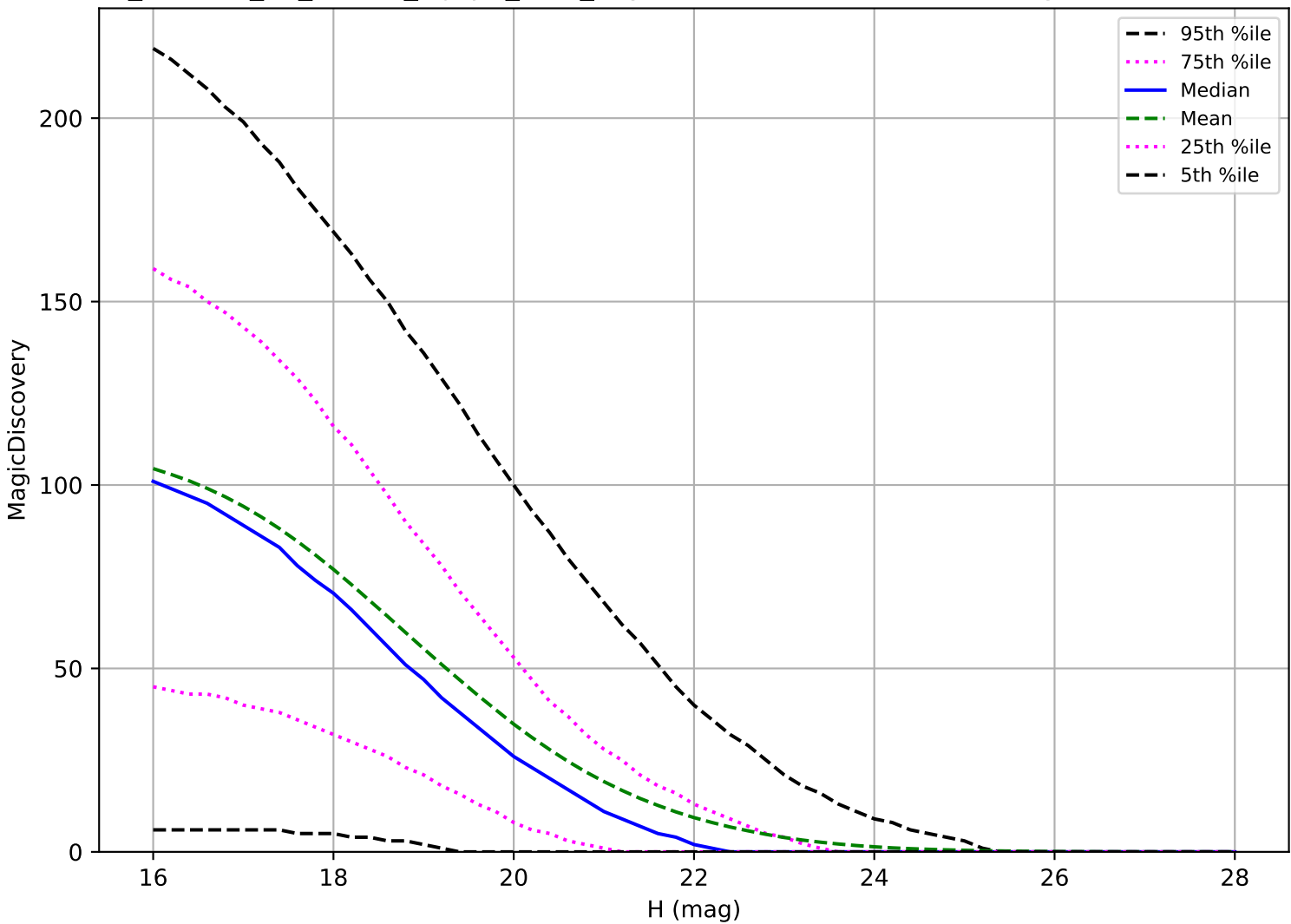
roll_uniform_eh_acc0.8_mjdp0_v3.4_10yrs: PHA 6 detections in 60 nights detection loss
