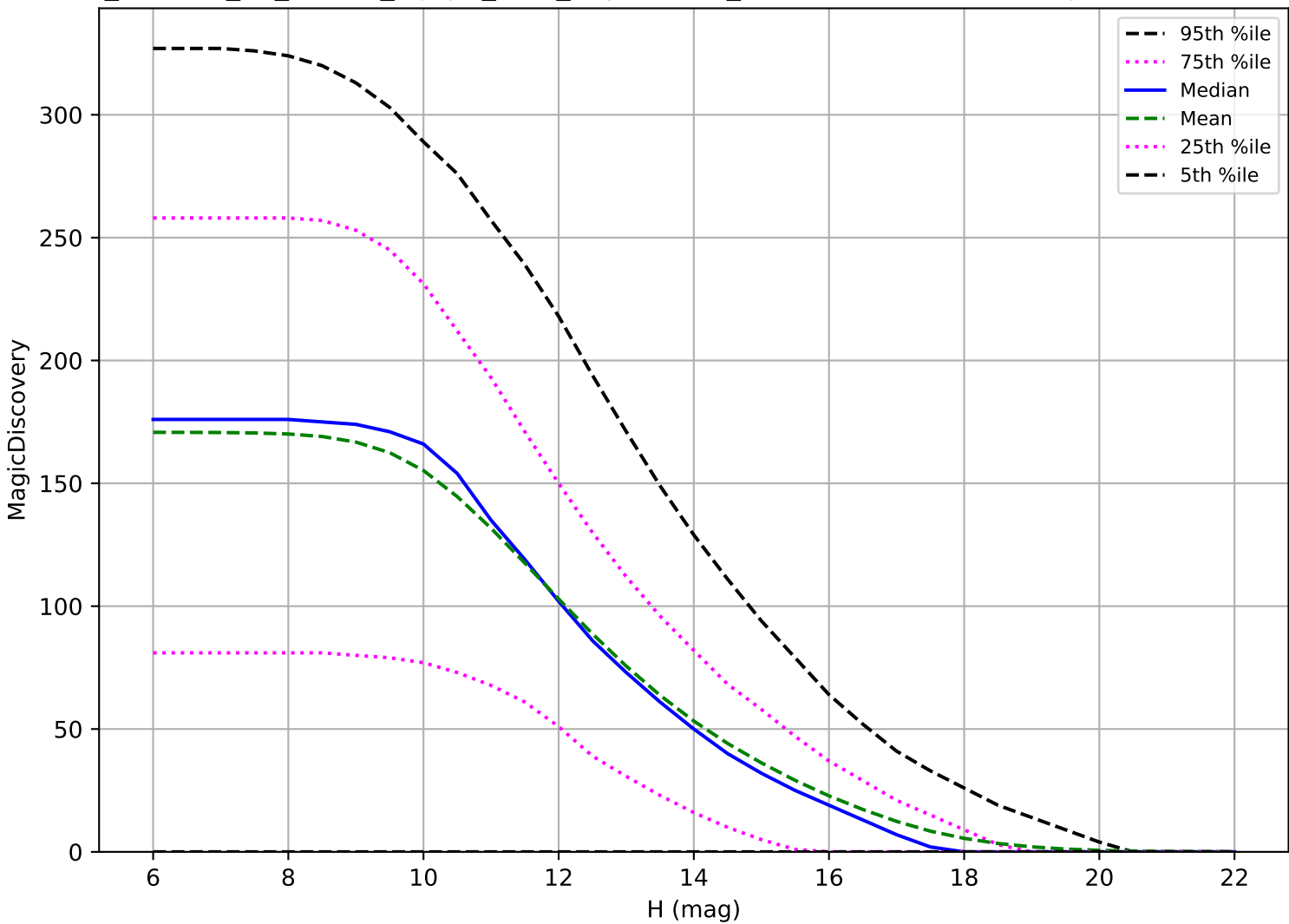
roll_uniform_eh_acc0.8_mjdp0_v3.4_10yrs: OCC_r5 6 detections in 60 nights detection loss
