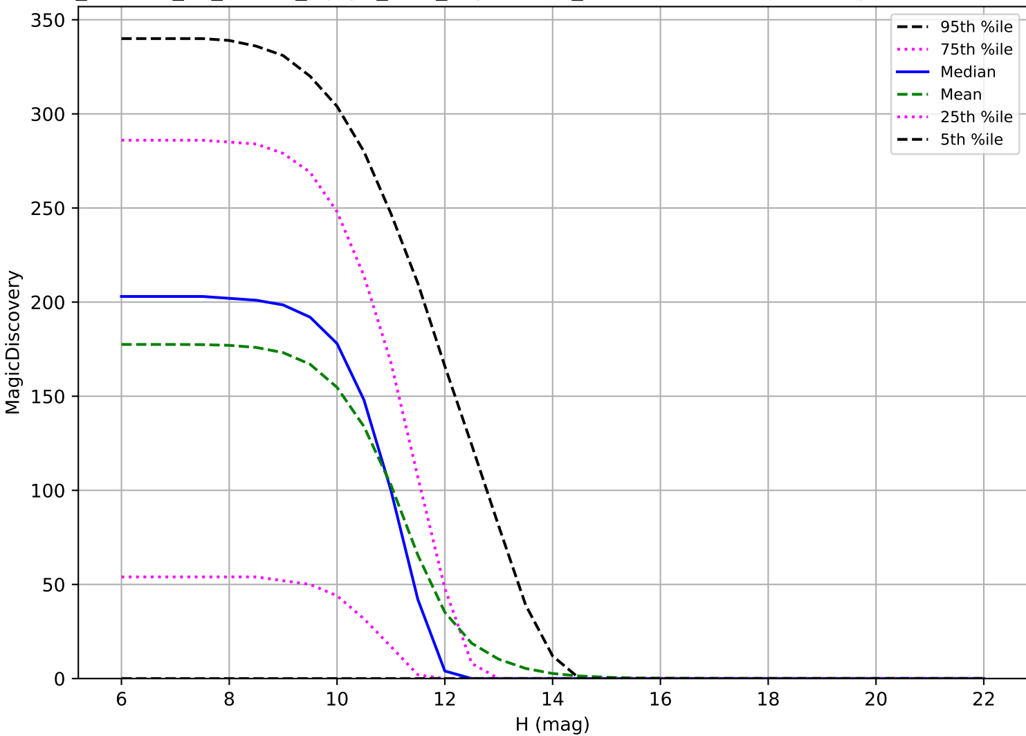
roll_uniform_eh_acc0.8_mjdp0_v3.4_10yrs: OCC_r20 6 detections in 60 nights detection loss
