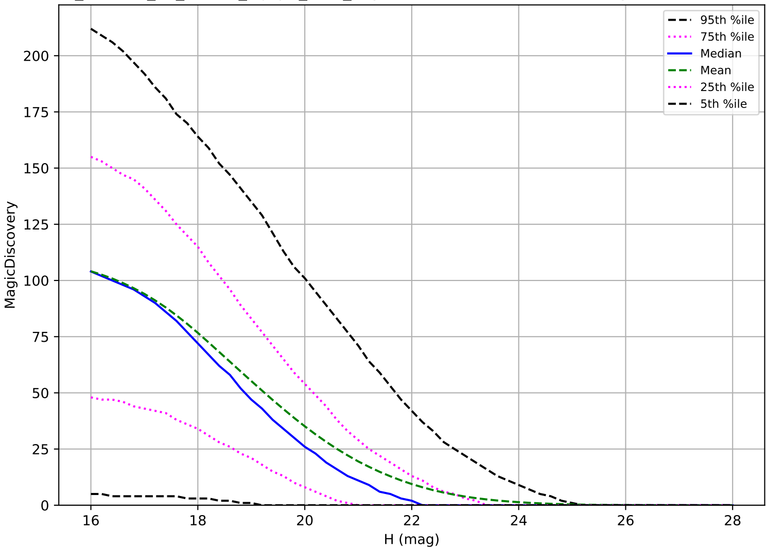
roll_uniform_eh_acc0.8_mjdp0_v3.4_10yrs: NEO 6 detections in 60 nights detection loss
