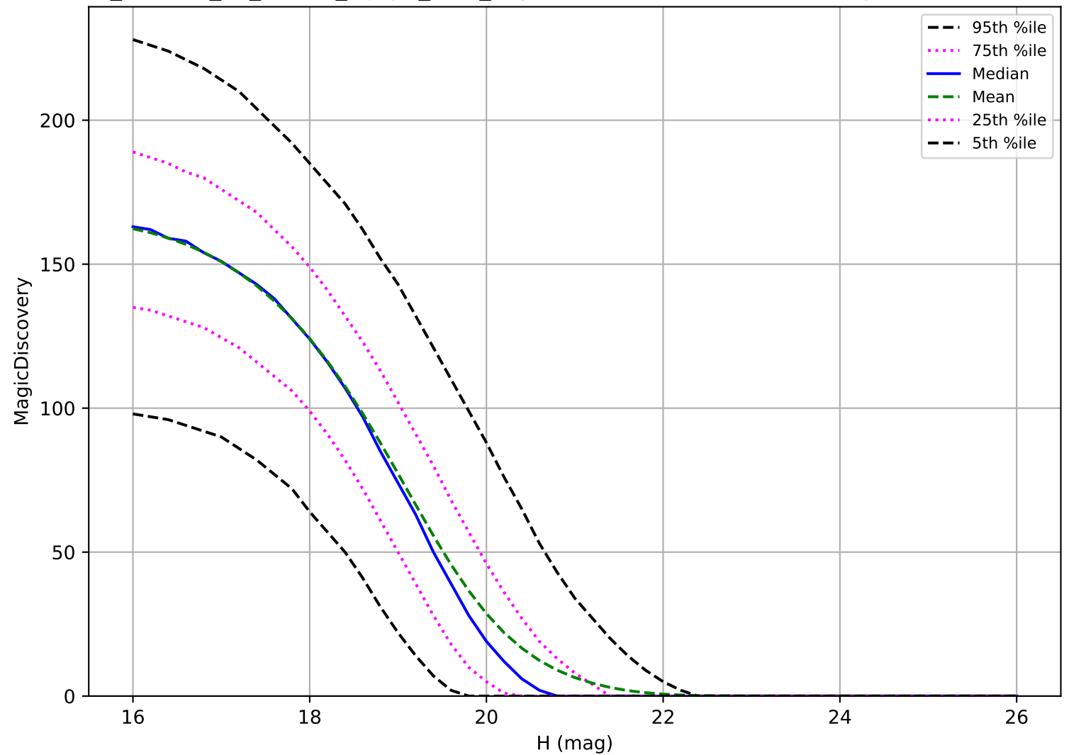
roll_uniform_eh_acc0.8_mjdp0_v3.4_10yrs: MBA 6 detections in 60 nights detection loss
