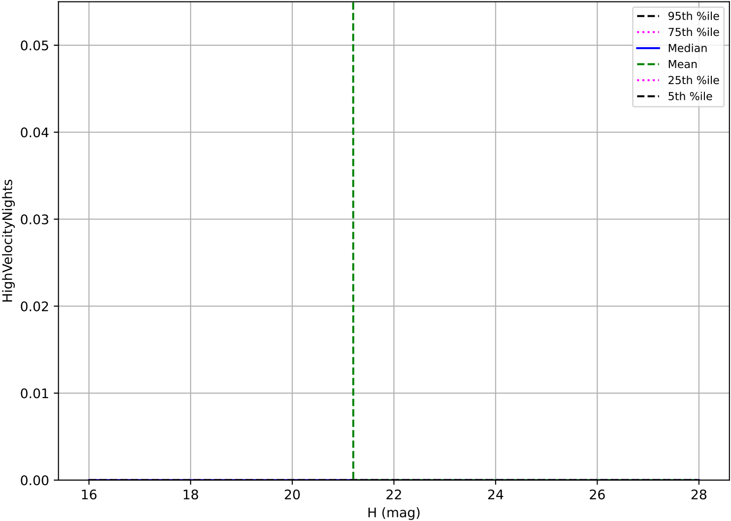
roll_uniform_eh_acc0.8_mjdp0_v3.4_10yrs: Vatira High velocity pair detection loss
