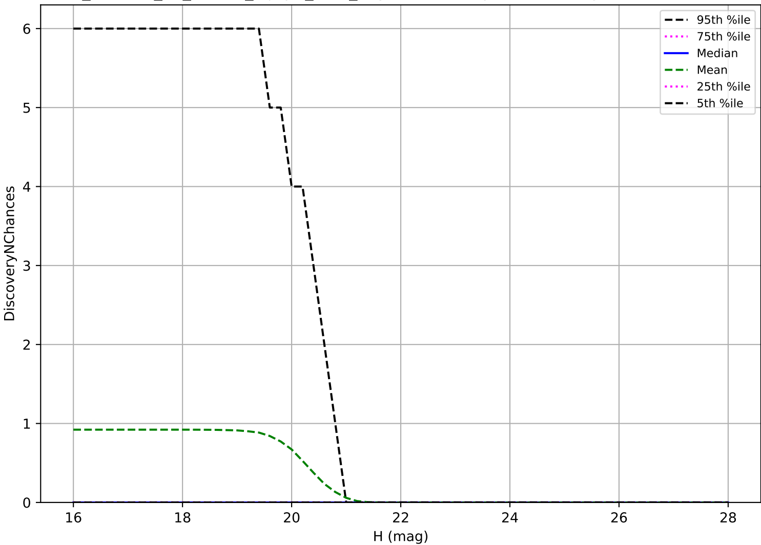
roll_uniform_eh_acc0.8_mjdp0_v3.4_10yrs: Vatira 3 pairs in 15 nights detection loss
