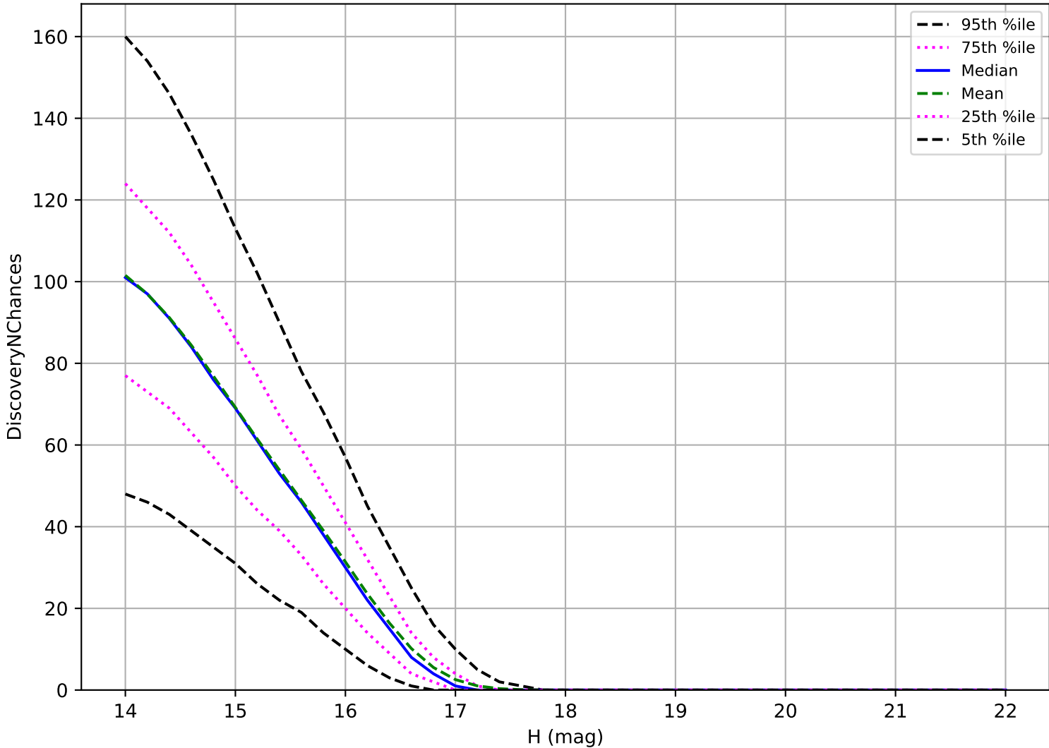
roll_uniform_eh_acc0.8_mjdp0_v3.4_10yrs: Trojan 3 pairs in 15 nights detection loss
