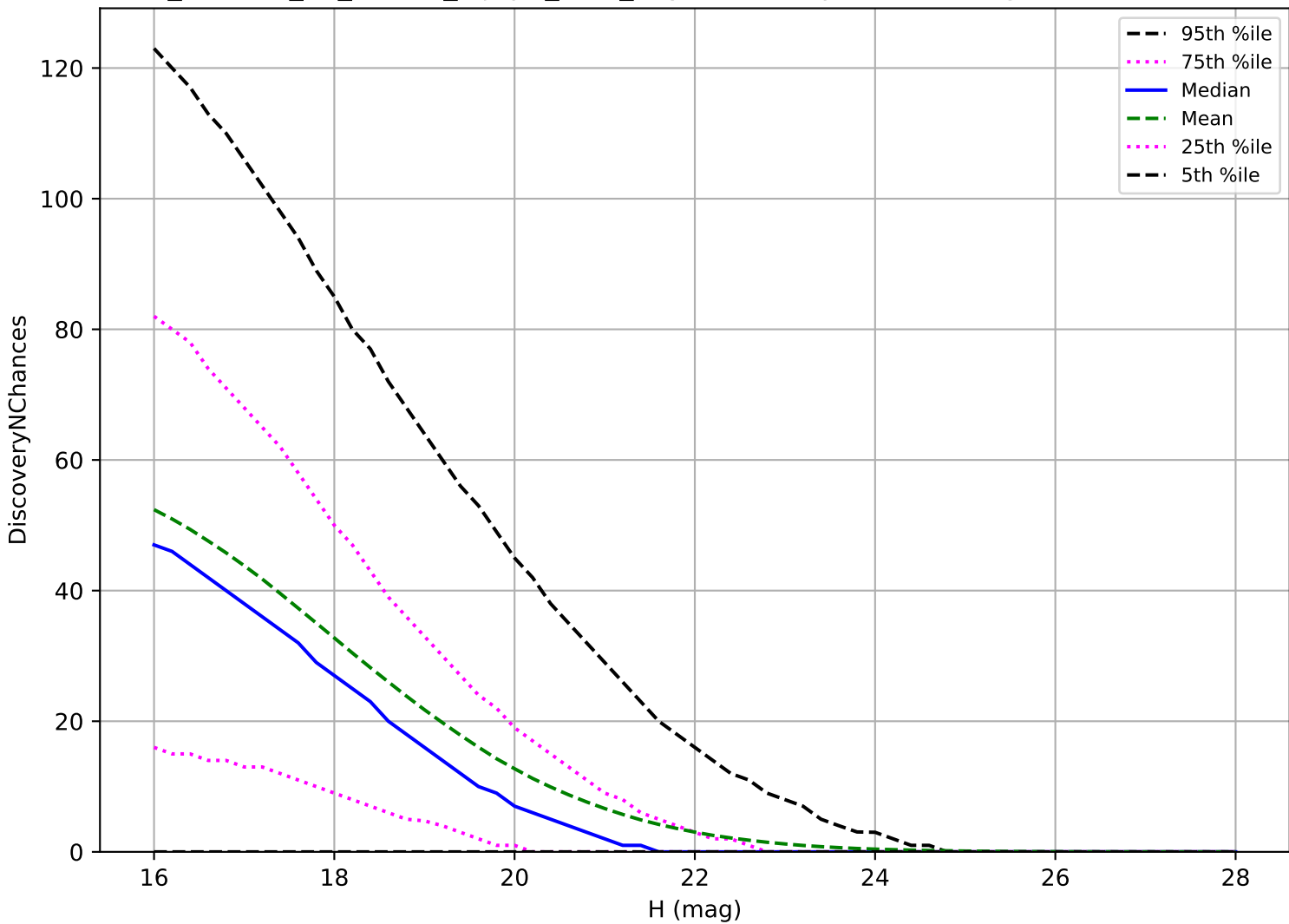
roll_uniform_eh_acc0.8_mjdp0_v3.4_10yrs: PHA 3 pairs in 15 nights detection loss
