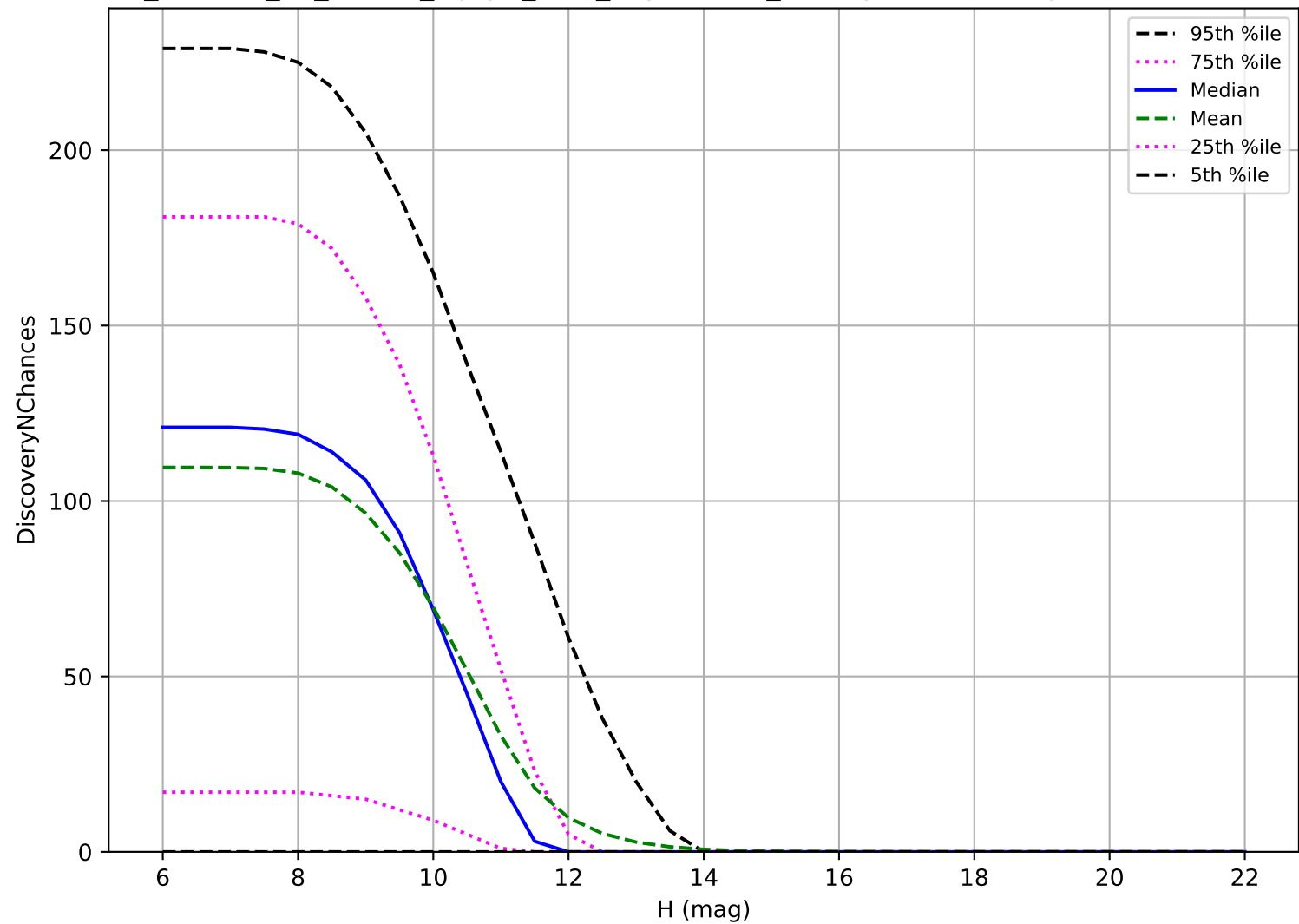
roll_uniform_eh_acc0.8_mjdp0_v3.4_10yrs: OCC_r20 3 pairs in 15 nights detection loss
