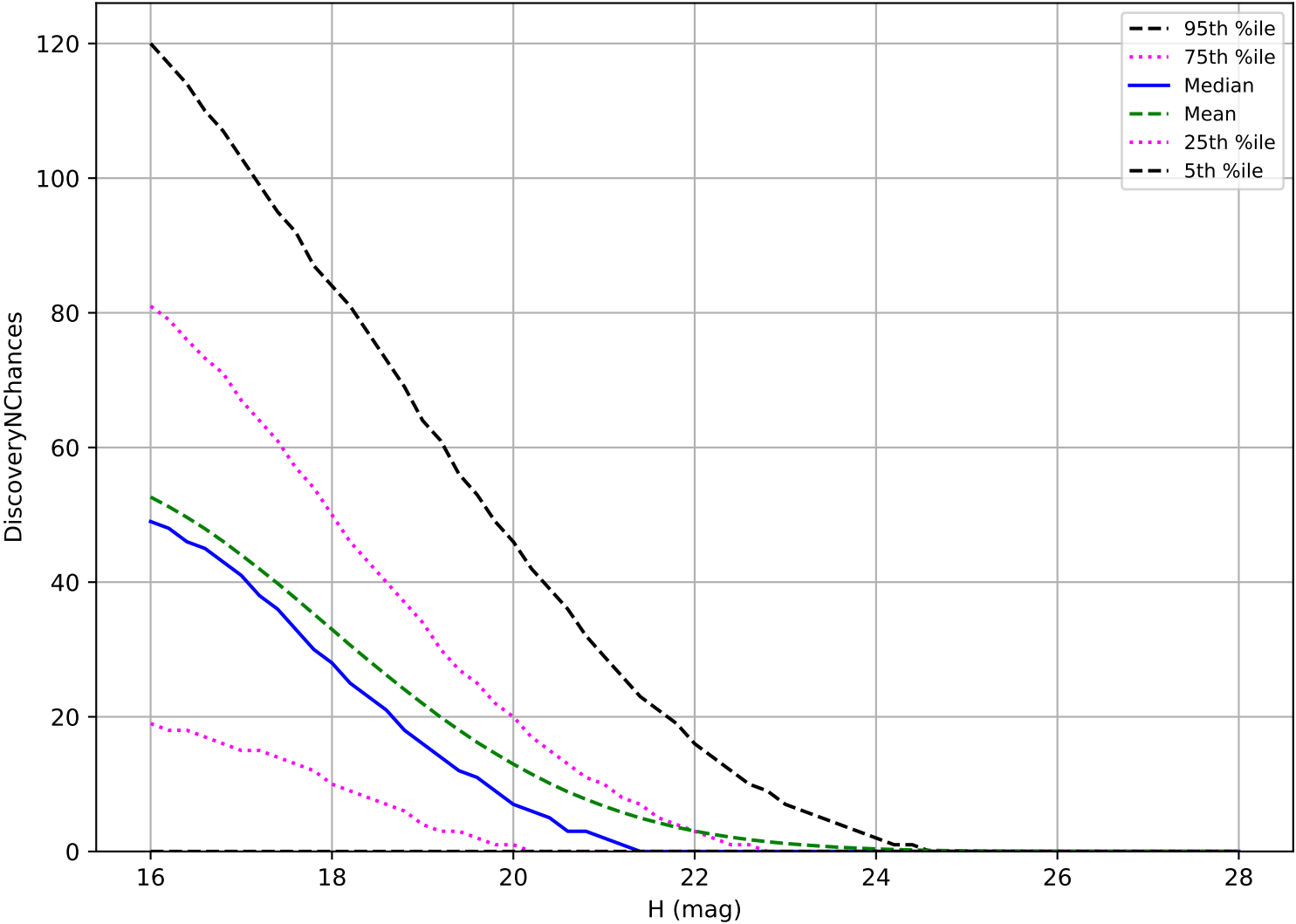
roll_uniform_eh_acc0.8_mjdp0_v3.4_10yrs: NEO 3 pairs in 15 nights detection loss
