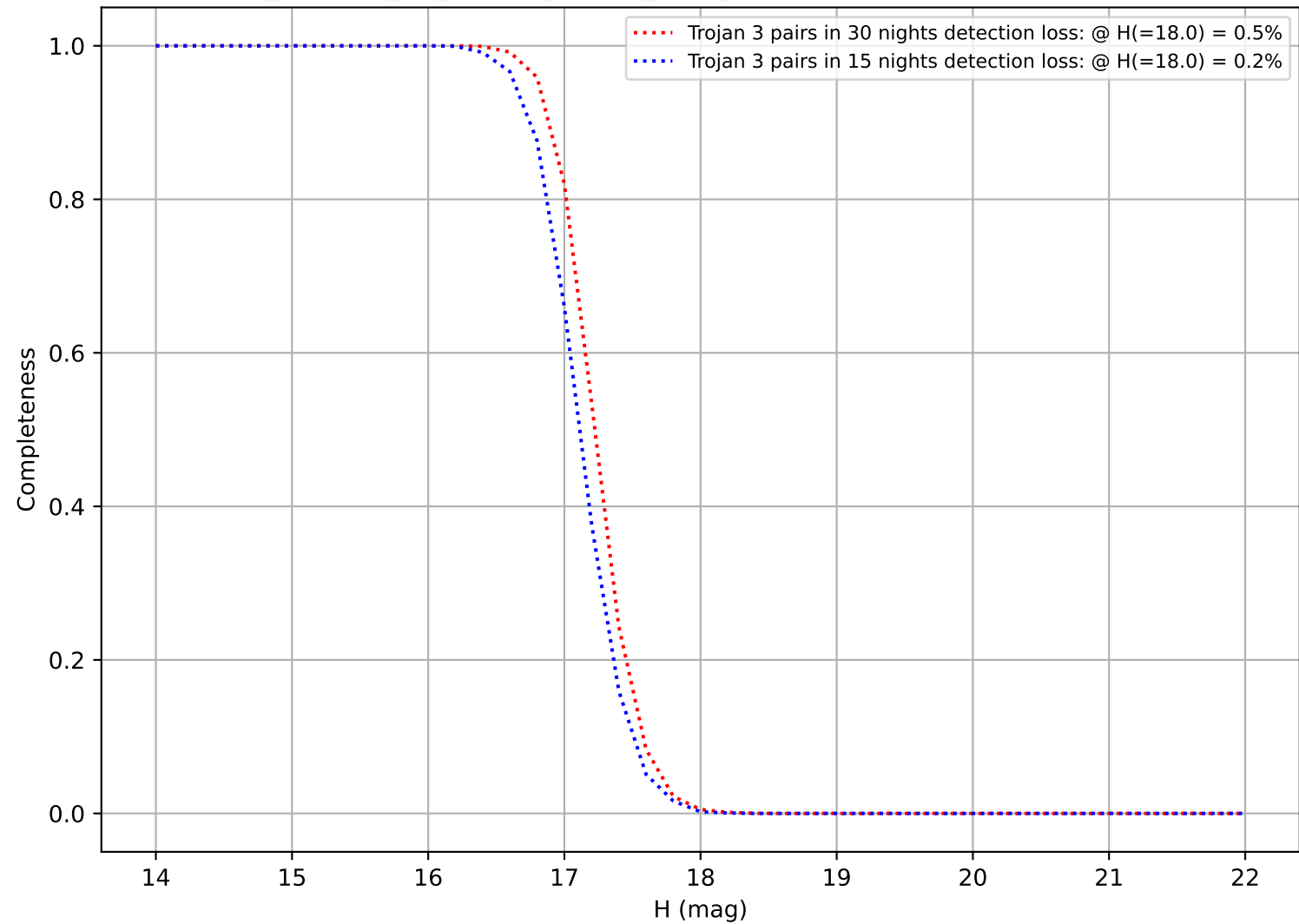
roll_uniform_eh_acc0.8_mjdp0_v3.4_10yrs: DifferentialCompleteness
