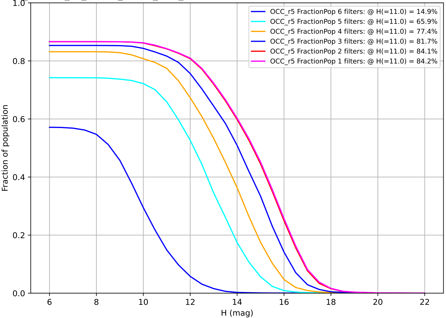
roll_uniform_eh_acc0.8_mjdp0_v3.4_10yrs: Fraction of population with colors in X filters OCC_r5
