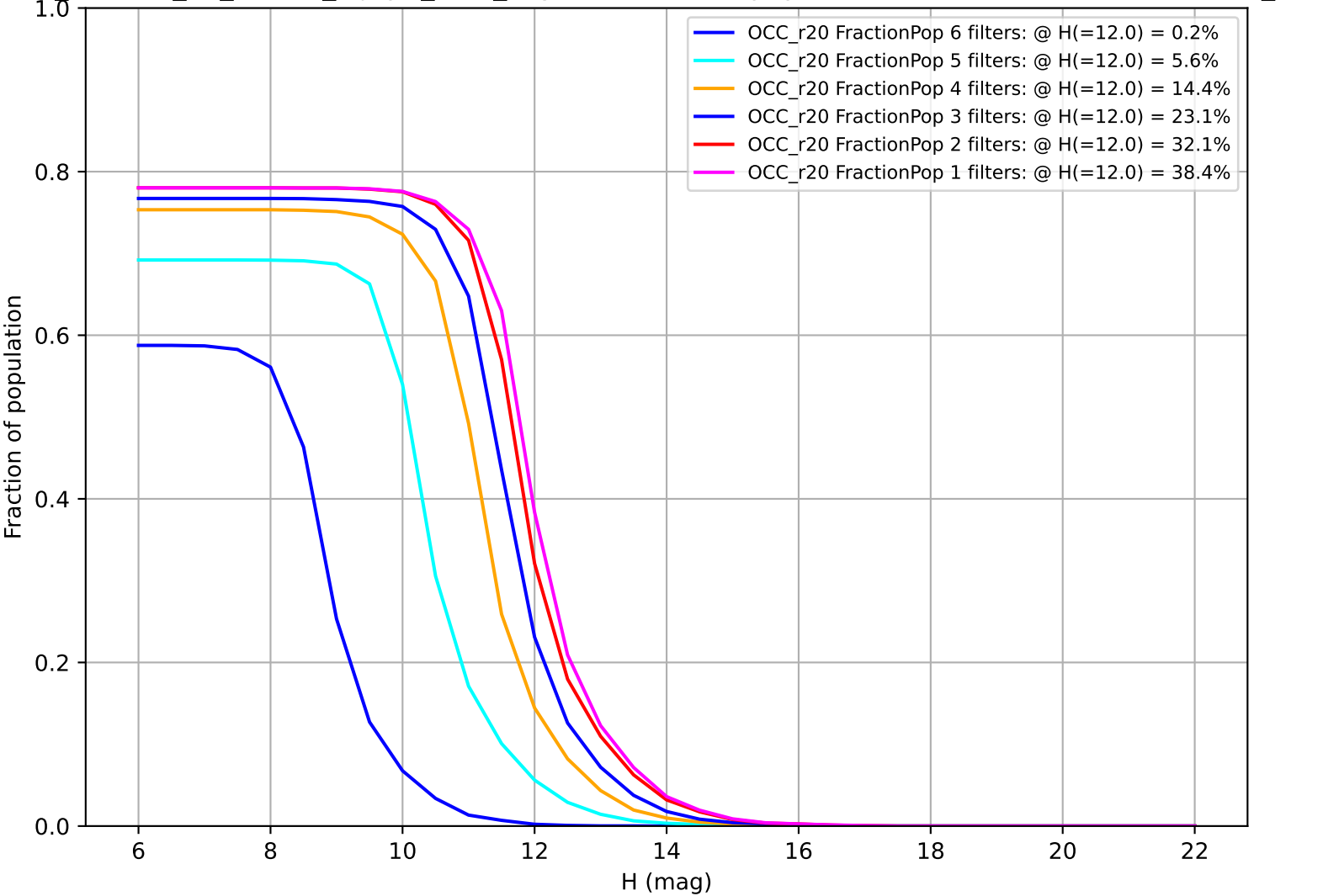
roll_uniform_eh_acc0.8_mjdp0_v3.4_10yrs: Fraction of population with colors in X filters OCC_r20
