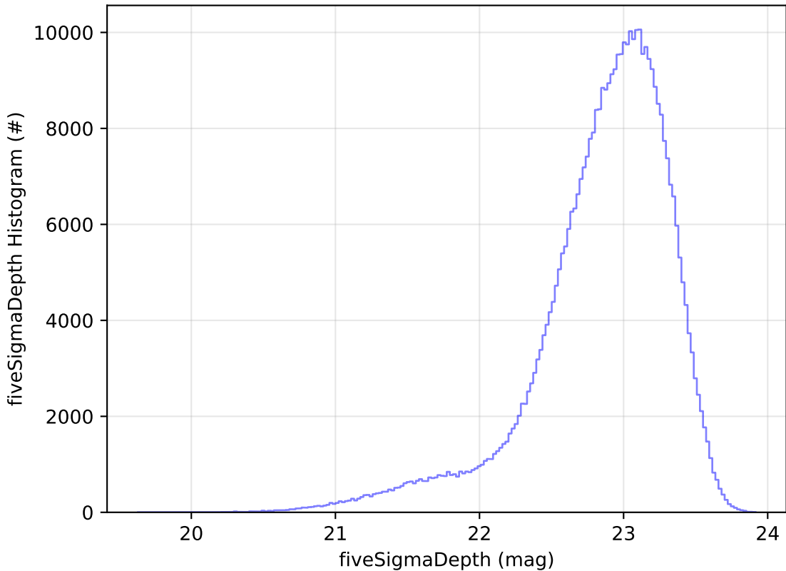
roll_uniform_eh_acc0.8_mjdp0_v3.4_10yrs z: fiveSigmaDepth Histogram
