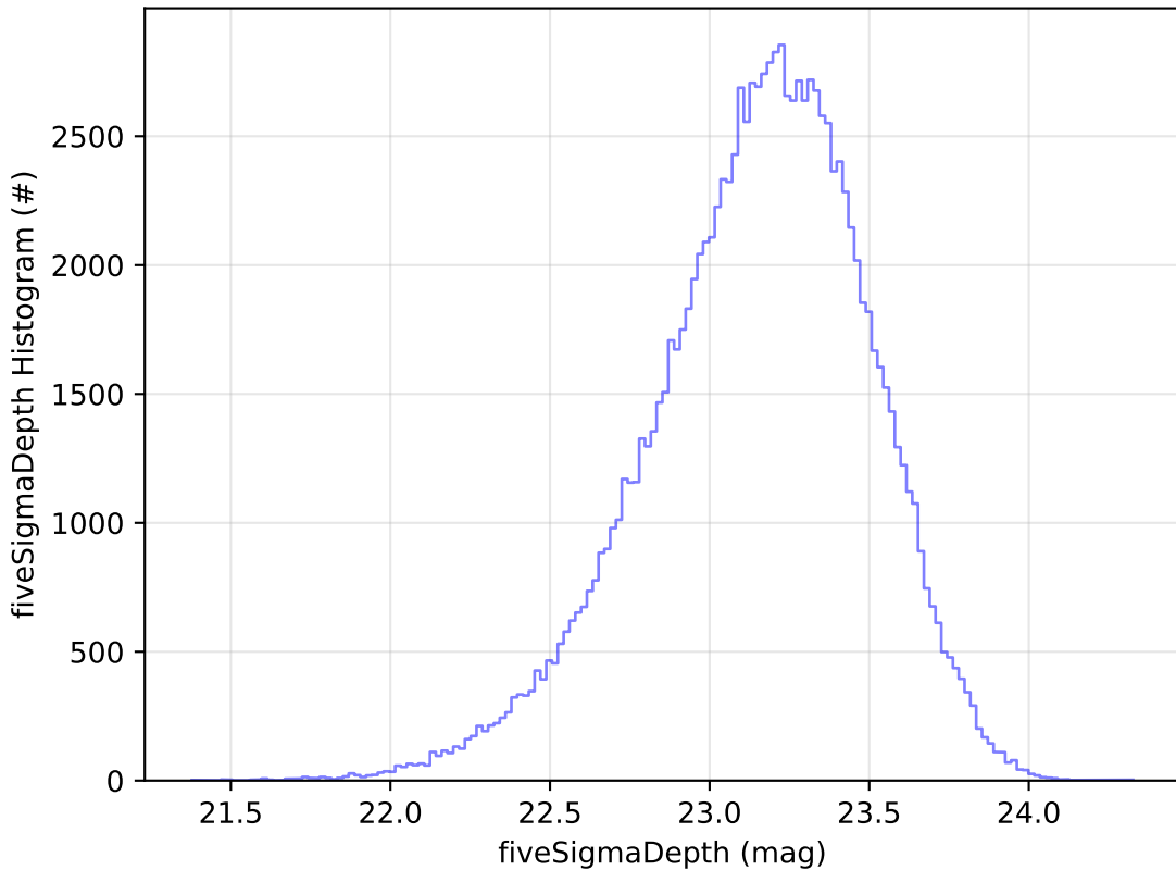
roll_uniform_eh_acc0.8_mjdp0_v3.4_10yrs u: fiveSigmaDepth Histogram
