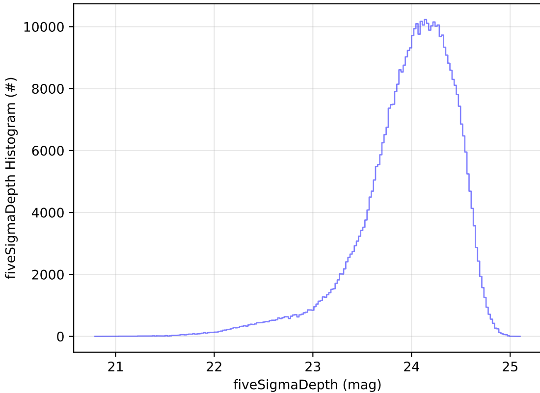
roll_uniform_eh_acc0.8_mjdp0_v3.4_10yrs r: fiveSigmaDepth Histogram
