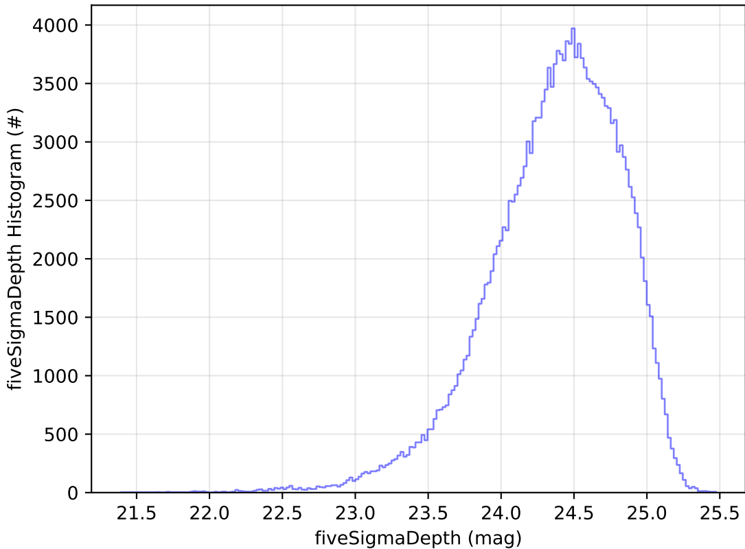
roll_uniform_eh_acc0.8_mjdp0_v3.4_10yrs g: fiveSigmaDepth Histogram
