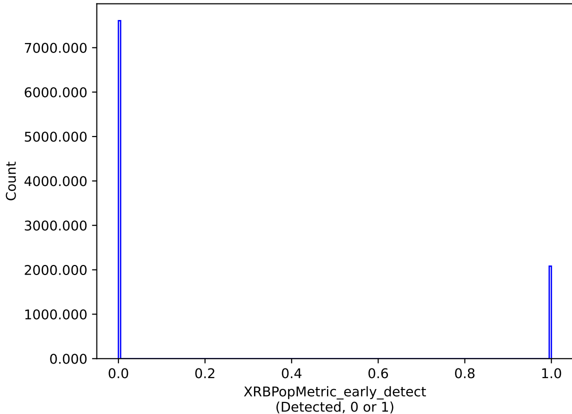
roll_uniform_eh_acc0.8_mjdp0_v3.4_10yrs : XRBPoMetric_early_detect
