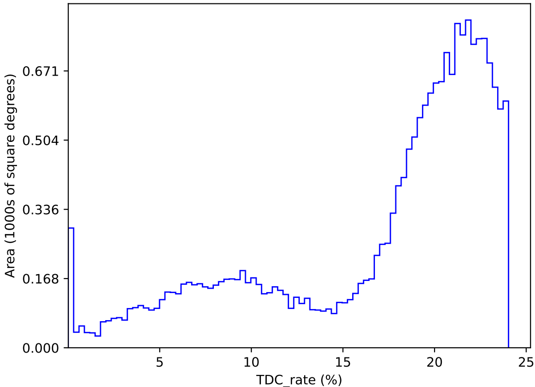
roll_uniform_eh_acc0.8_mjdp0_v3.4_10yrs : TDC_rate
