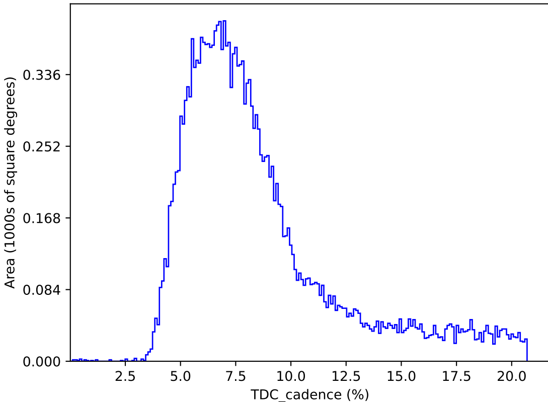
roll_uniform_eh_acc0.8_mjdp0_v3.4_10yrs : TDC_cadence
