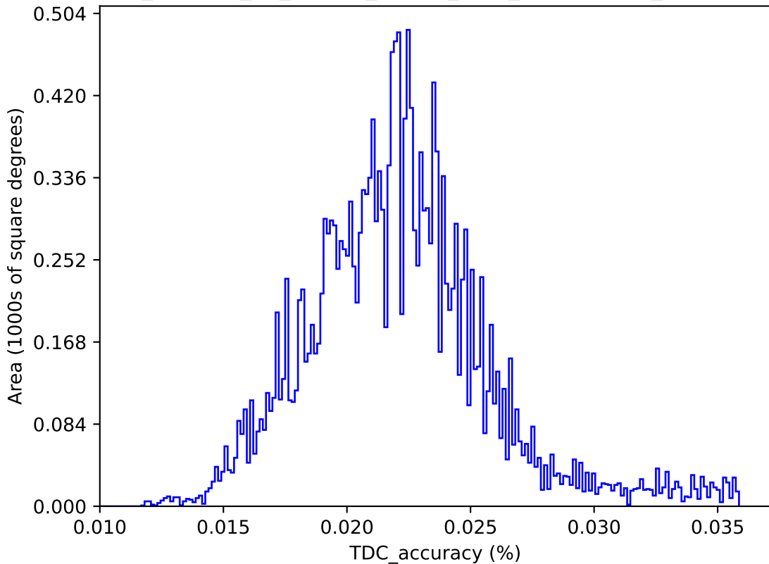
roll_uniform_eh_acc0.8_mjdp0_v3.4_10yrs : TDC_accuracy
