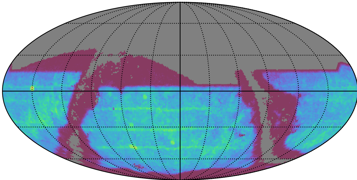
roll_uniform_eh_acc0.8_mjdp0_v3.4_10yrs : SNSLMetric
