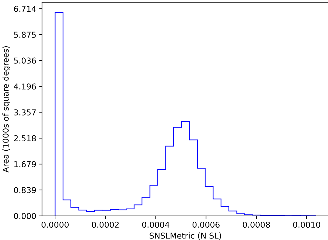
roll_uniform_eh_acc0.8_mjdp0_v3.4_10yrs : SNSLMetric
