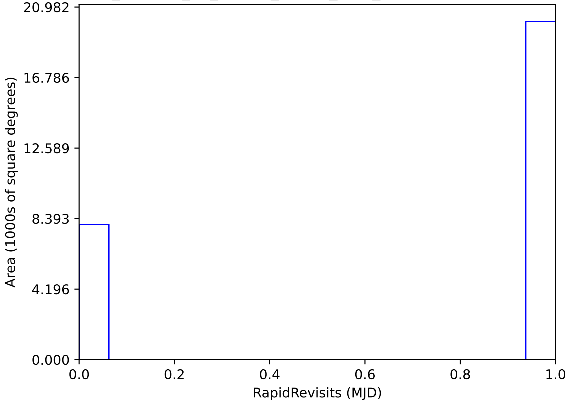
roll_uniform_eh_acc0.8_mjdp0_v3.4_10yrs : RapidRevisits
