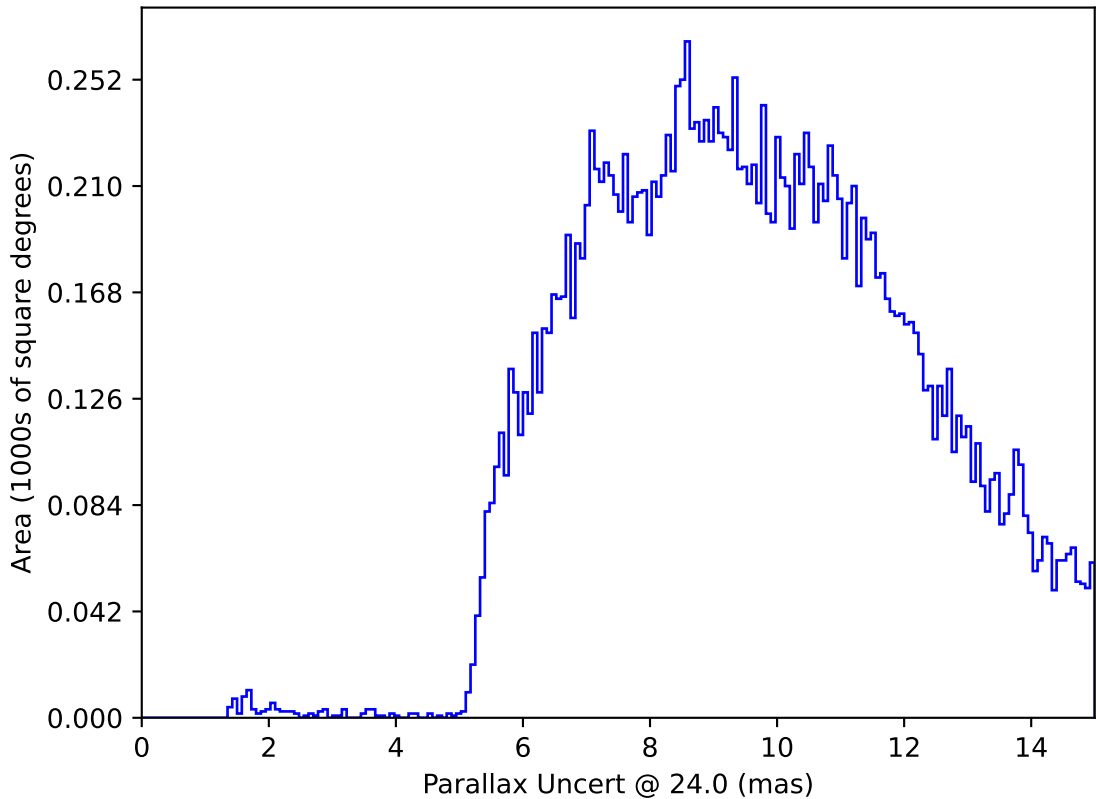
roll_uniform_eh_acc0.8_mjdp0_v3.4_10yrs : Parallax Uncert @ 24.0
