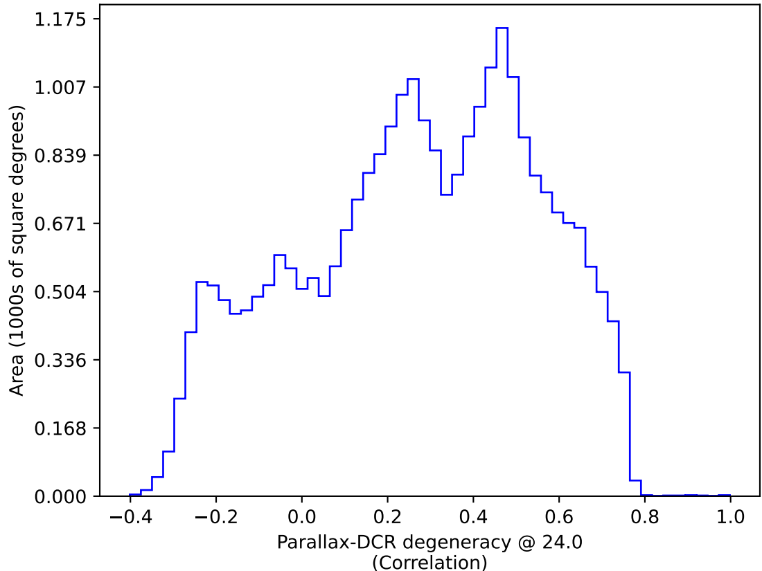
roll_uniform_eh_acc0.8_mjdp0_v3.4_10yrs : Parallax-DCR degeneracy @ 24.0
