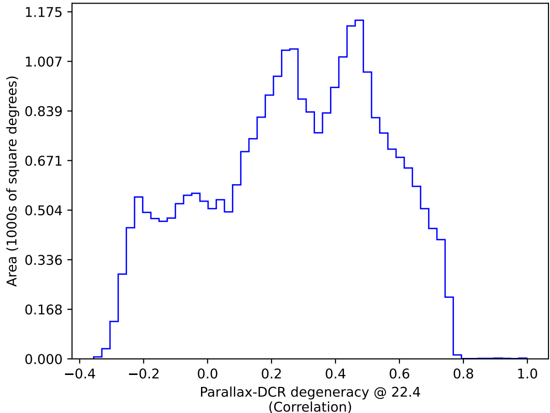
roll_uniform_eh_acc0.8_mjdp0_v3.4_10yrs : Parallax-DCR degeneracy @ 22.4
