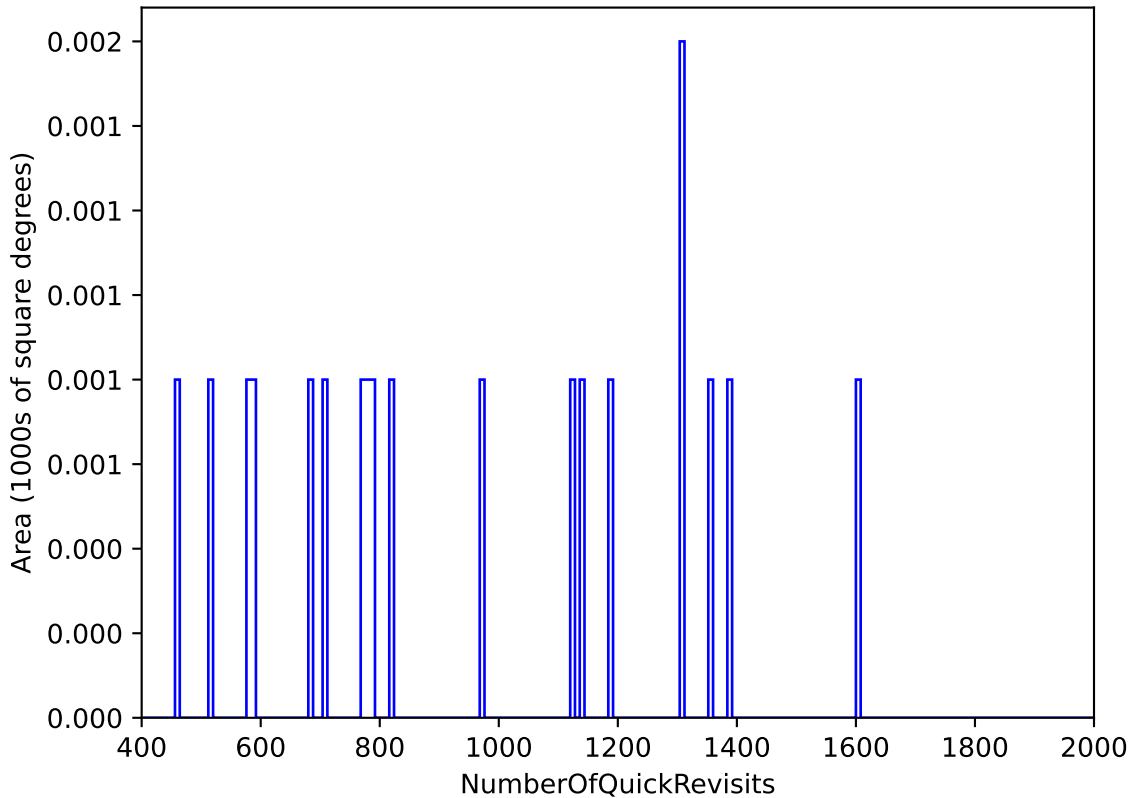
roll_uniform_eh_acc0.8_mjdp0_v3.4_10yrs : NumberOfQuickRevisits
