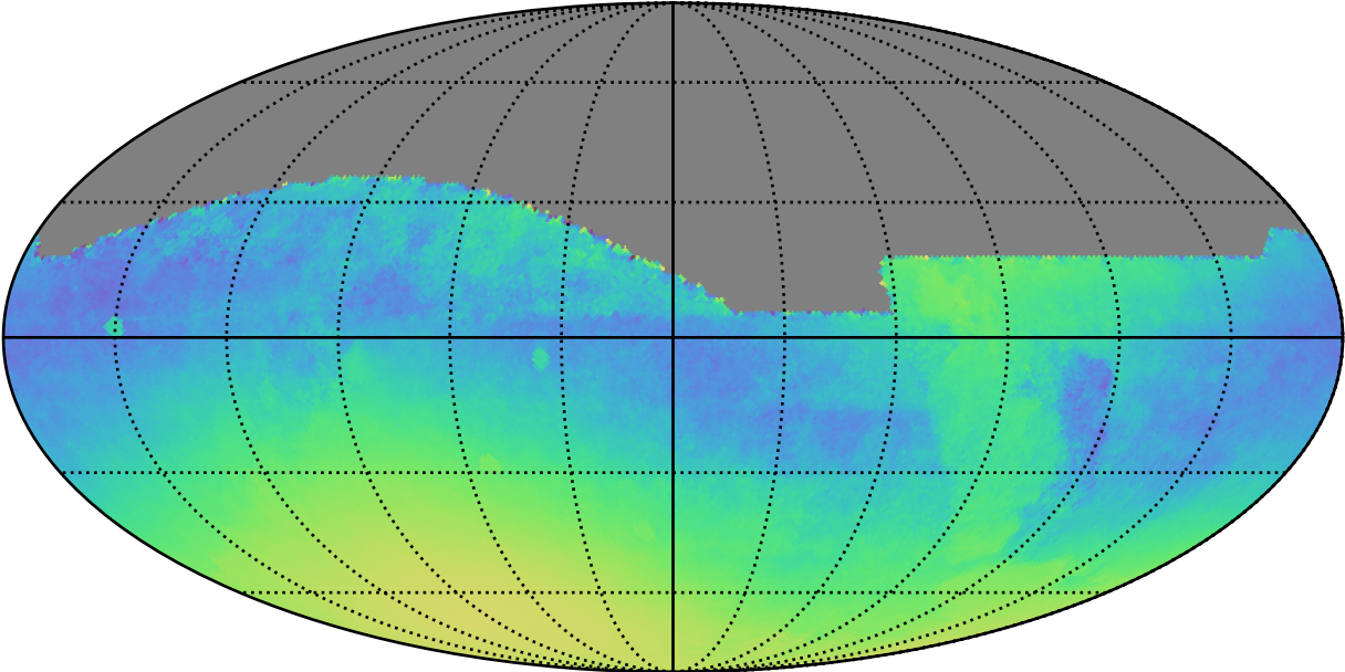
roll_uniform_eh_acc0.8_mjdp0_v3.4_10yrs : Normalized Parallax Uncert @ 24.0
