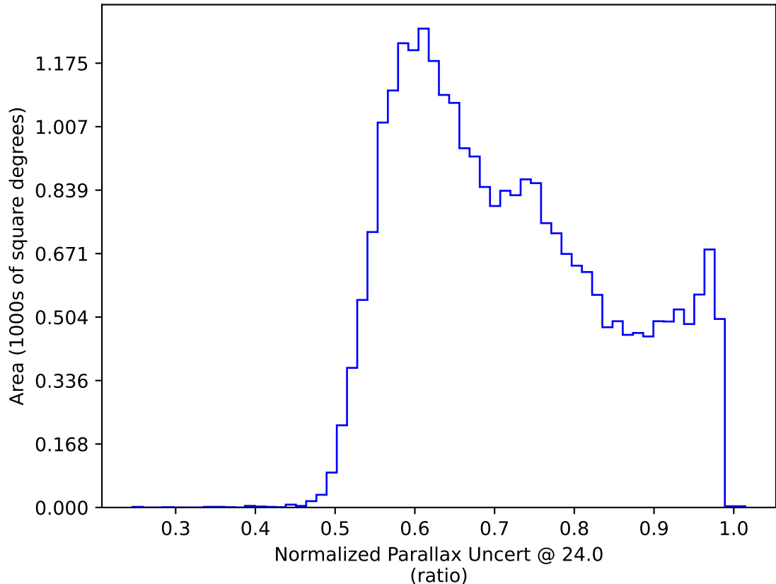
roll_uniform_eh_acc0.8_mjdp0_v3.4_10yrs : Normalized Parallax Uncert @ 24.0
