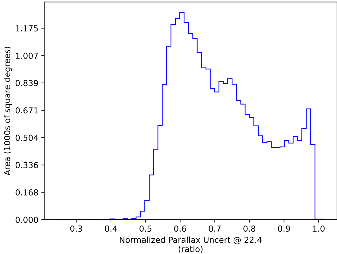
roll_uniform_eh_acc0.8_mjdp0_v3.4_10yrs : Normalized Parallax Uncert @ 22.4
